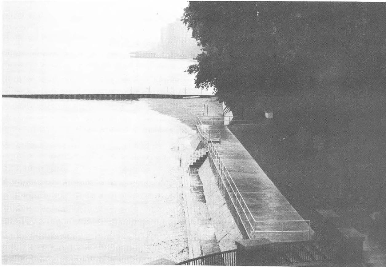
Figure 7. A seawall at Kenilworth, Illinois, has successfully stabilized the bank.
